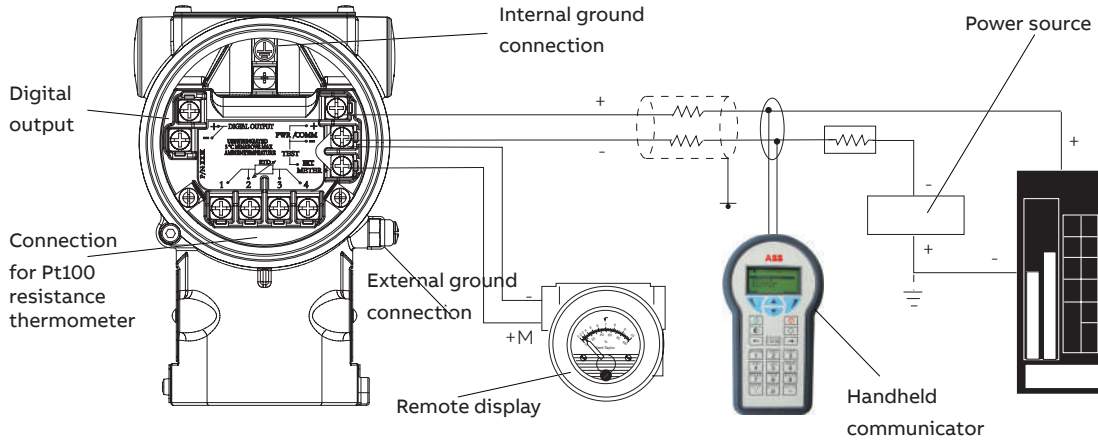
Figure 9: Electrical connections
